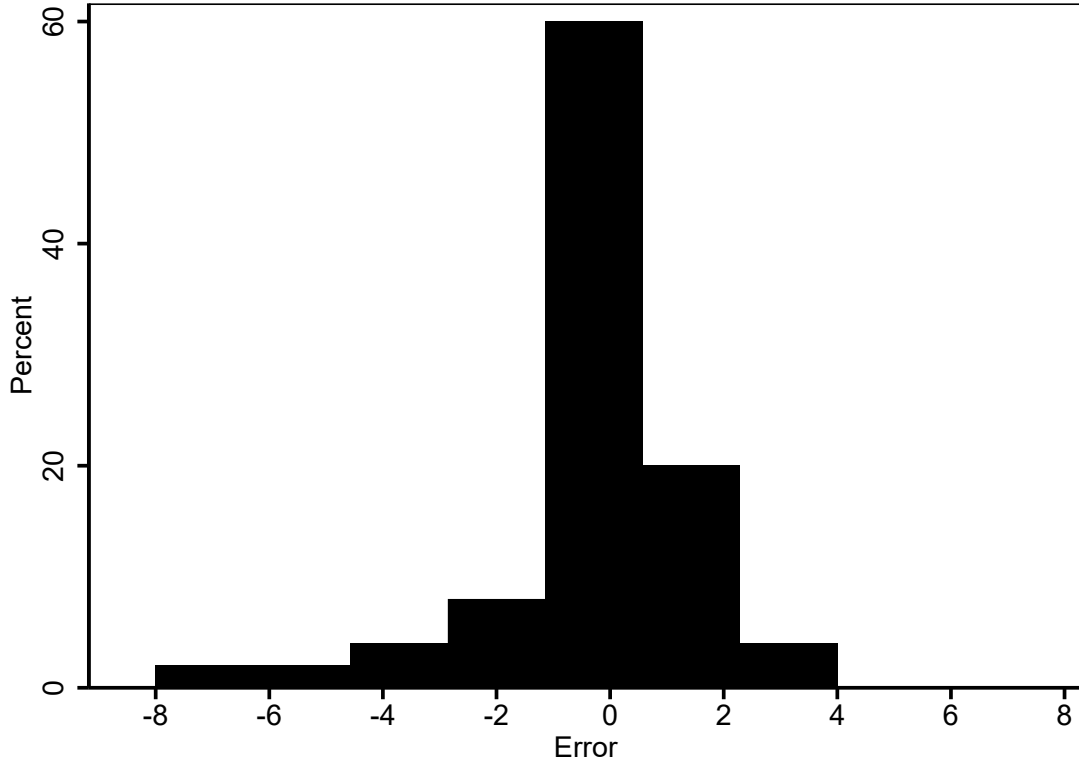
Figure 2: Error Distribution
